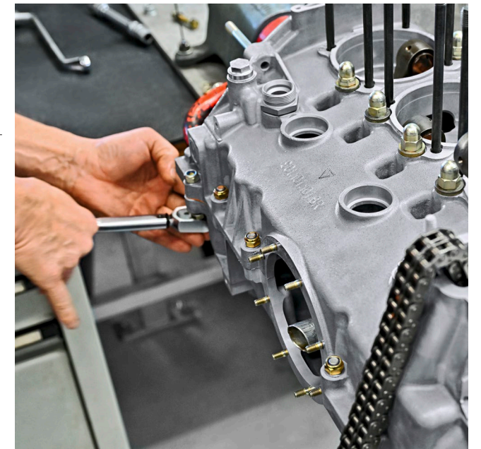
Crankcase, magnesium, 2.7 L Part no. 91110100145 911 F model (1973), only for 911 Carrera RS 2.7 911 G model (1974–1977), only for vehicles with 2.7 L engines
