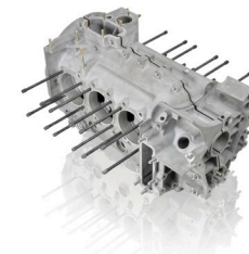
Crankcase, magnesium, 2.7 L Part no. 91110100145 911 F model (1973), only for 911 Carrera RS 2.7 911 G model (1974–1977), only for vehicles with 2.7 L engines
