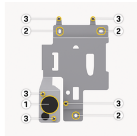
Fig. 12: Mounting plate
