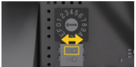
Fig. 55: Interruptor DIP
