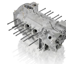
Magnesium crankcase 2.4 L Part no. 90110100147 911 F model (1972–1973), only for vehicles with 2.4 L engine
