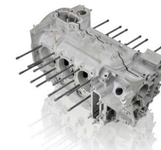
Magnesium crankcase 2.7 L Part no. 91110100145 911 F model (1973), only for 911 Carrera RS 2.7 911 G model (1974–1977), only for vehicles with 2.7 L engines
