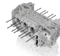
Magnesium crankcase 2.0/2.2 L Part no. 90110100146 911 F model (1968–1971), only for vehicles with 2.0 or 2.2 L engines
