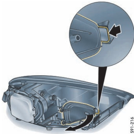
更换静态弯道灯灯泡 (H7, 55W)
